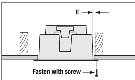
Fig. 3: Joist clearances
